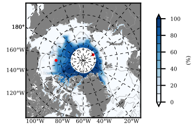
NSIDC mean SICON m09 2014
