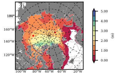
NSIDC mean SICON m03 2014
