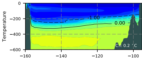
DFS52NEM405 / Beaufort Section 1979
