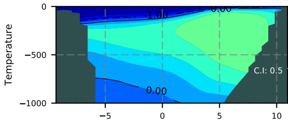
DFS52NEM405 / FramS Section 1983
