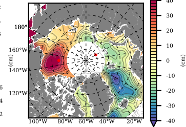
Mean DOT from Armitage et al. 2017 2011
