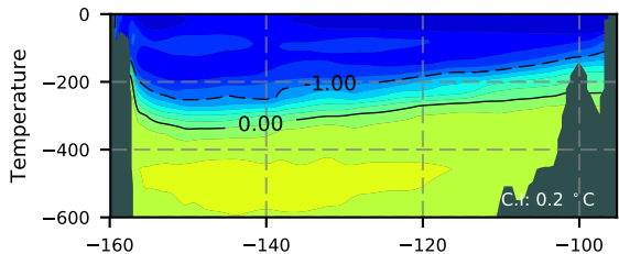
ERA01NEM405 / Beaufort Section 1980
