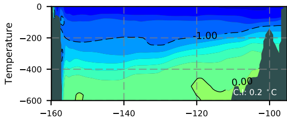
ERA01NEM405 / Beaufort Section 2012
