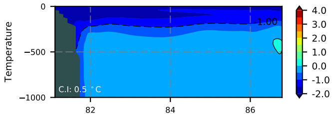
ERA01NEM405 / Kara Section 2003
