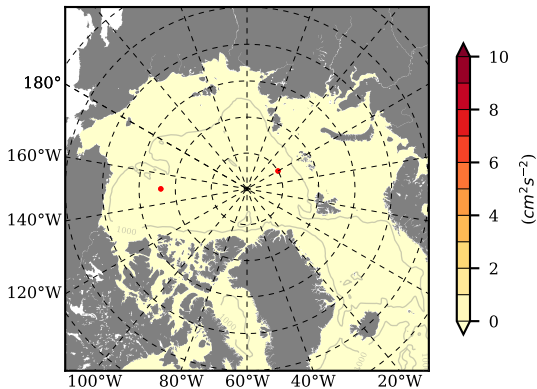
ERA01NEM405ALB mean EKE @ 0 m over 1984
