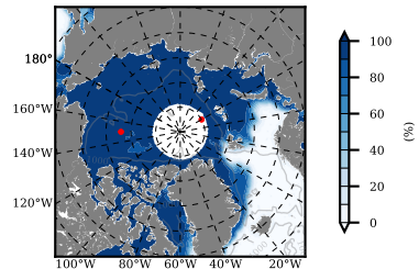
NSIDC mean SICON m09 1986
