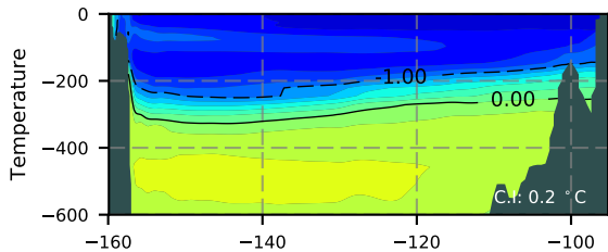
ERA01NEM405ALB / Beaufort Section 1979
