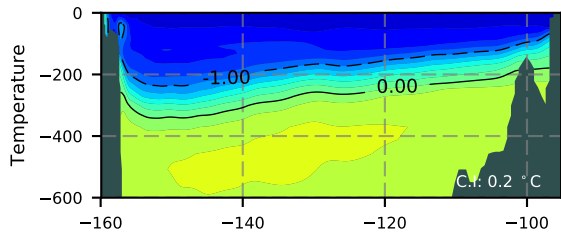
ERA01NEM405ALB / Beaufort Section 1987
