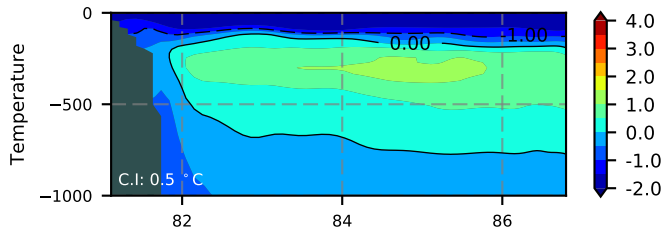
ERA01NEM405ALB / Kara Section 1980
