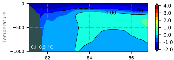
ERA01NEM405ALB / Kara Section 1986
