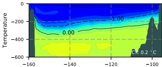
ERA01NEM405ALL / Beaufort Section 1981
