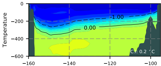
ERA01NEM405ALL / Beaufort Section 1983
