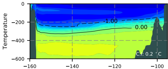
ERA01NEM405ASC / Beaufort Section 1979
