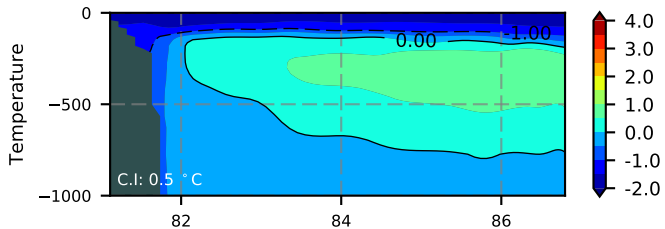
ERA01NEM405ASC / Kara Section 1982
