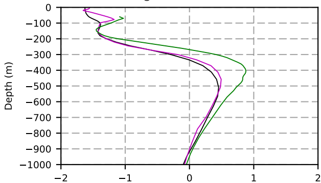
1984 mean temperature @ moor Arctic B box
