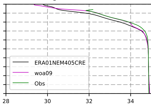
1984 mean Salinity @ moor Arctic B box
