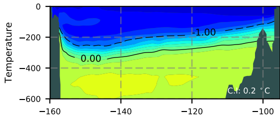
ERA01NEM405CRE / Beaufort Section 1981
