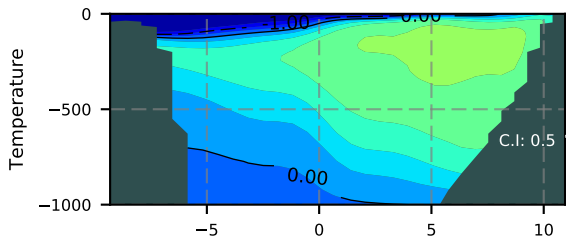
ERA01NEM405CRE / FramS Section 1984
