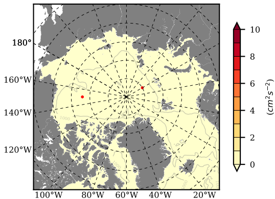
ERA01NEM405LAS mean EKE @ 0 m over 1983
