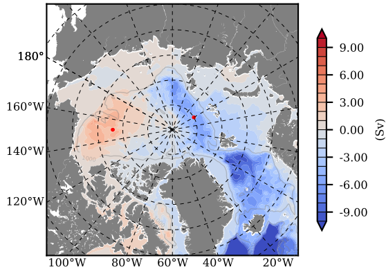
mean PSI over 1986
