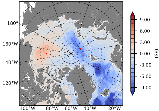
mean PSI over 1988
