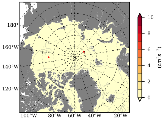
ERA01NEM405LAS mean EKE @ 0 m over 1996
