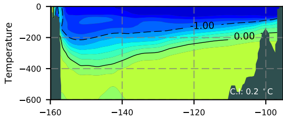
ERA01NEM405LAS / Beaufort Section 1997
