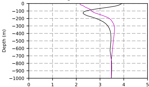
1979 mean temperature @ moor BRAVO box
