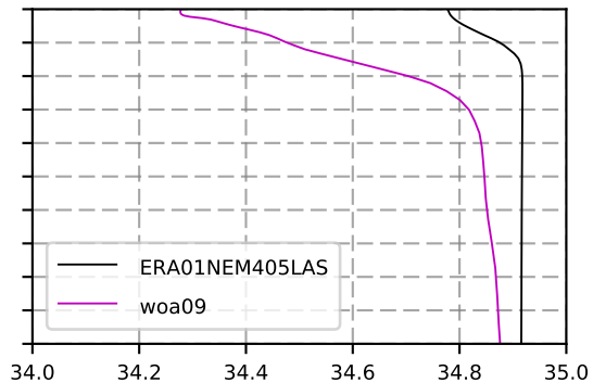
1993 mean Salinity @ moor BRAVO box
