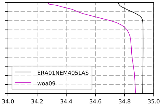
1995 mean Salinity @ moor BRAVO box
