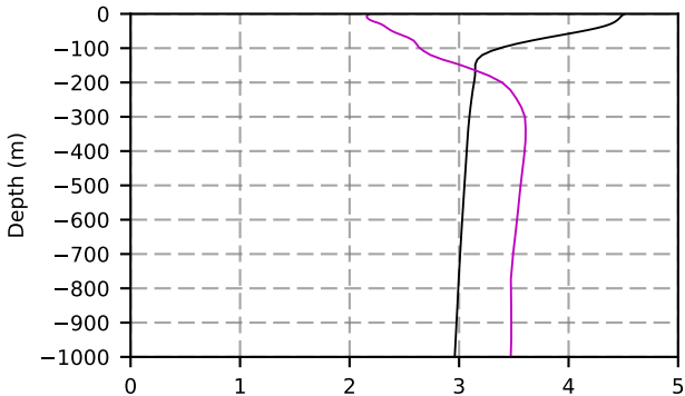
1995 mean temperature @ moor BRAVO box
