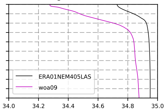
1998 mean Salinity @ moor BRAVO box
