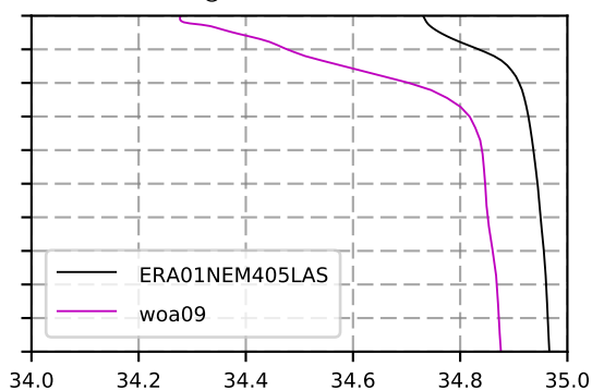
1999 mean Salinity @ moor BRAVO box
