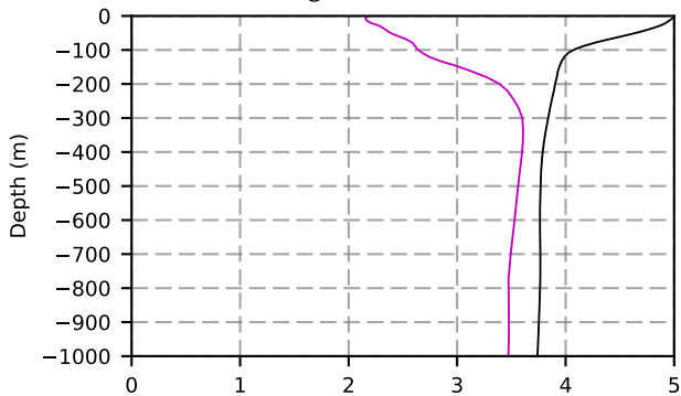
1999 mean temperature @ moor BRAVO box
