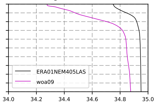
2000 mean Salinity @ moor BRAVO box
