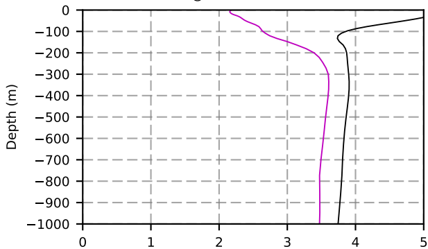
2003 mean temperature @ moor BRAVO box
