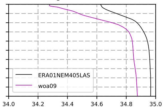
2003 mean Salinity @ moor BRAVO box
