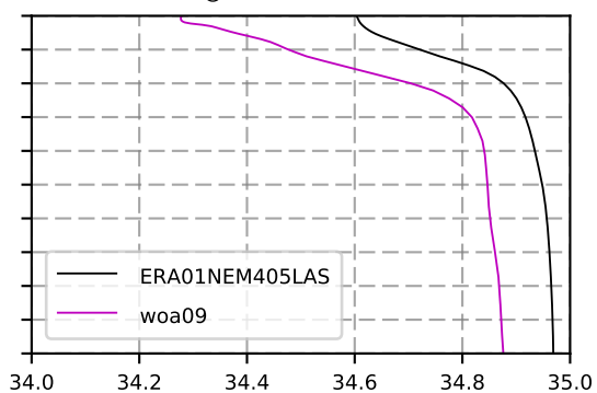
2004 mean Salinity @ moor BRAVO box
