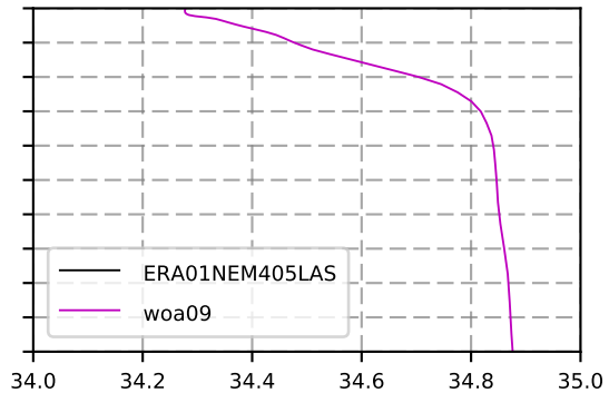
2005 mean Salinity @ moor BRAVO box
