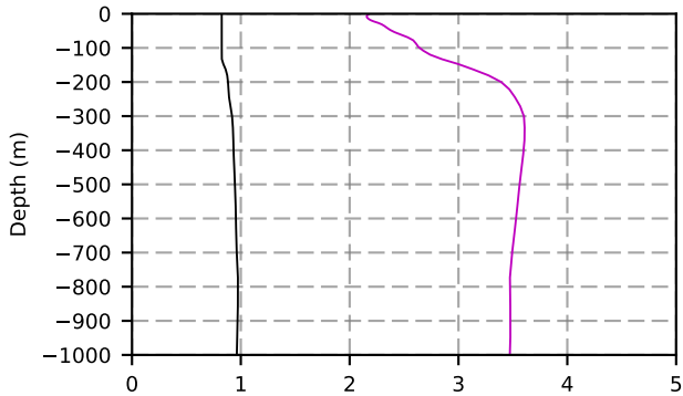
2005 mean temperature @ moor BRAVO box
