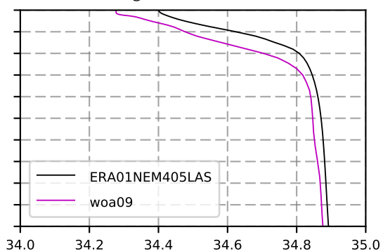
2008 mean Salinity @ moor BRAVO box
