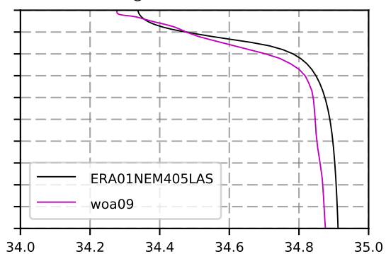
2009 mean Salinity @ moor BRAVO box
