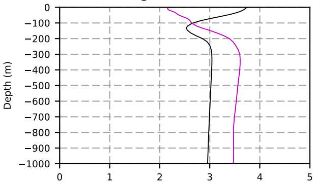
1984 mean temperature @ moor BRAVO box
