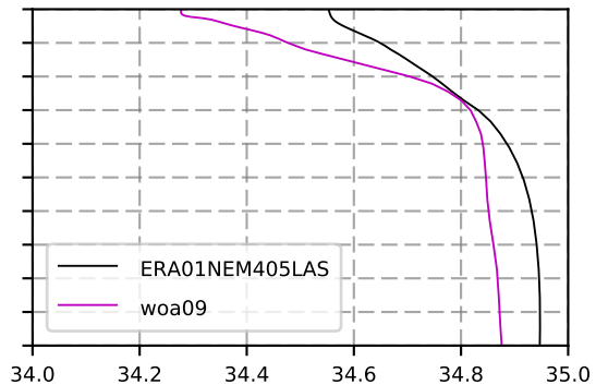
1988 mean Salinity @ moor BRAVO box
