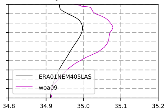
1986 mean Salinity @ moor GIN seas box
