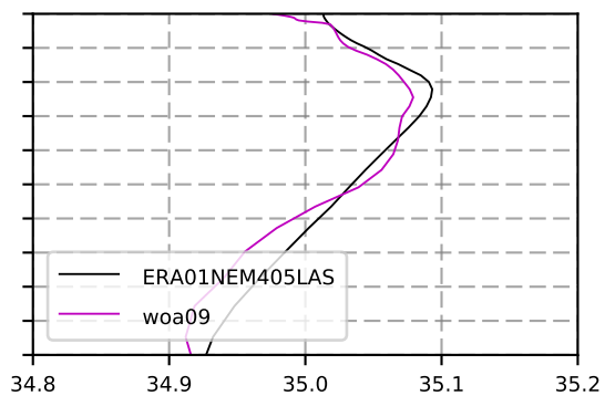
1989 mean Salinity @ moor GIN seas box
