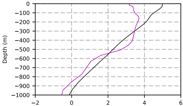
1989 mean temperature @ moor GIN seas box
