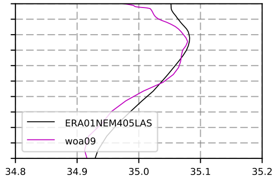
1990 mean Salinity @ moor GIN seas box
