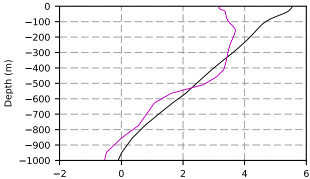
1990 mean temperature @ moor GIN seas box
