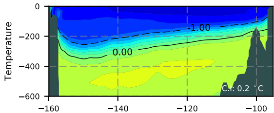
ERA01NEM405LAS / Beaufort Section 1985
