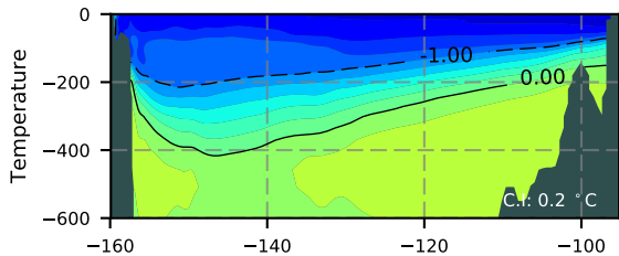
ERA01NEM405LAS / Beaufort Section 2000
