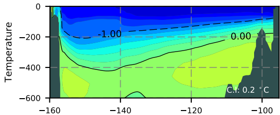
ERA01NEM405LAS / Beaufort Section 2004
