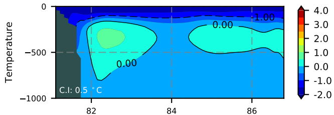
ERA01NEM405LAS / Kara Section 1993
