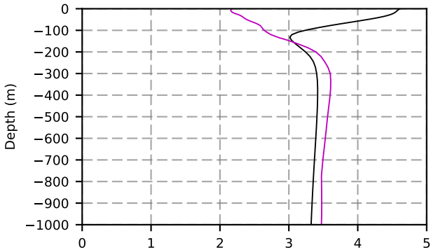
1981 mean temperature @ moor BRAVO box
