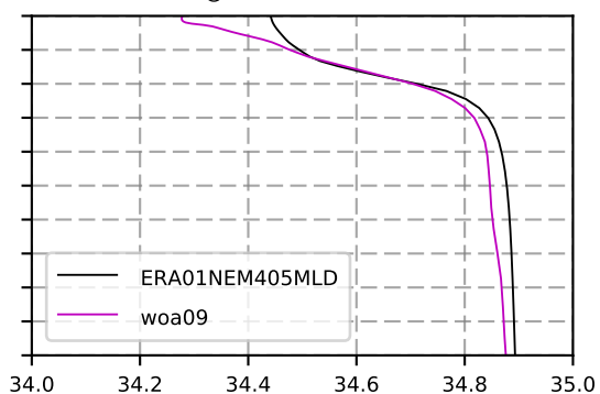
1982 mean Salinity @ moor BRAVO box
