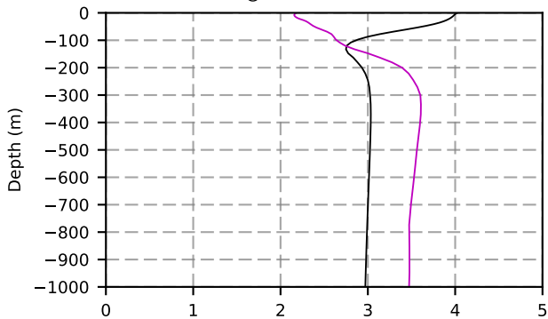
1984 mean temperature @ moor BRAVO box
