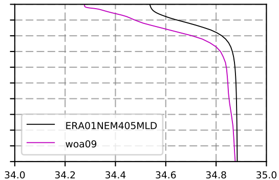
1984 mean Salinity @ moor BRAVO box
