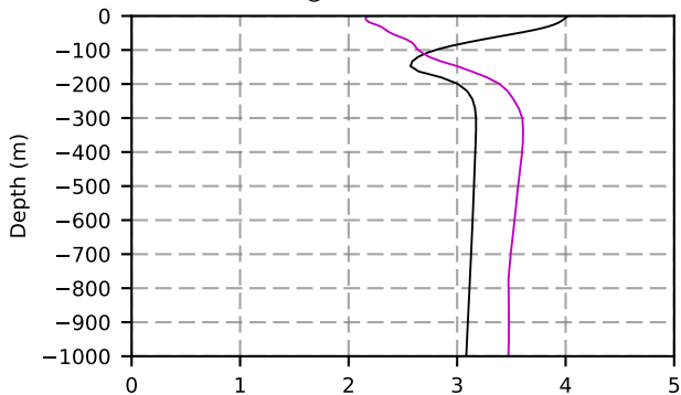
1985 mean temperature @ moor BRAVO box
