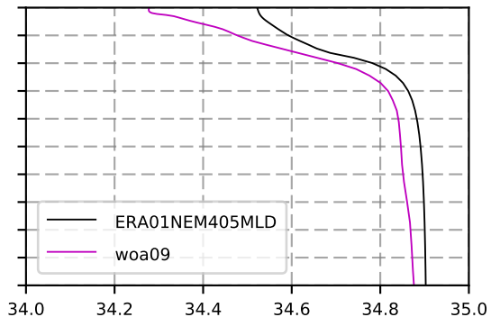
1985 mean Salinity @ moor BRAVO box
