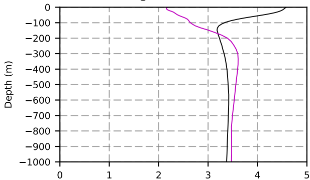
1989 mean temperature @ moor BRAVO box
