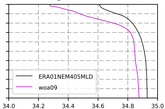
1989 mean Salinity @ moor BRAVO box
